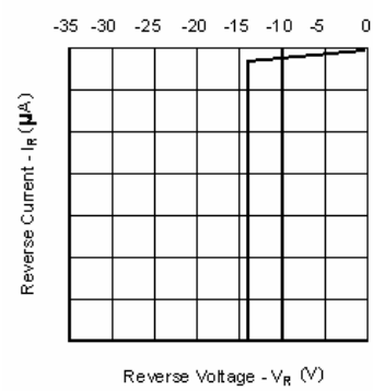
Figure 4-b: Reverse Voltage vs. Reverse Current – Blue and Green
